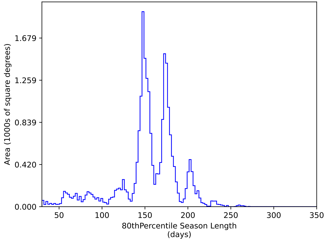
too_elab_r256_d2_griz_v3.4_10yrs All sky y band: 80thPercentile Season Length
