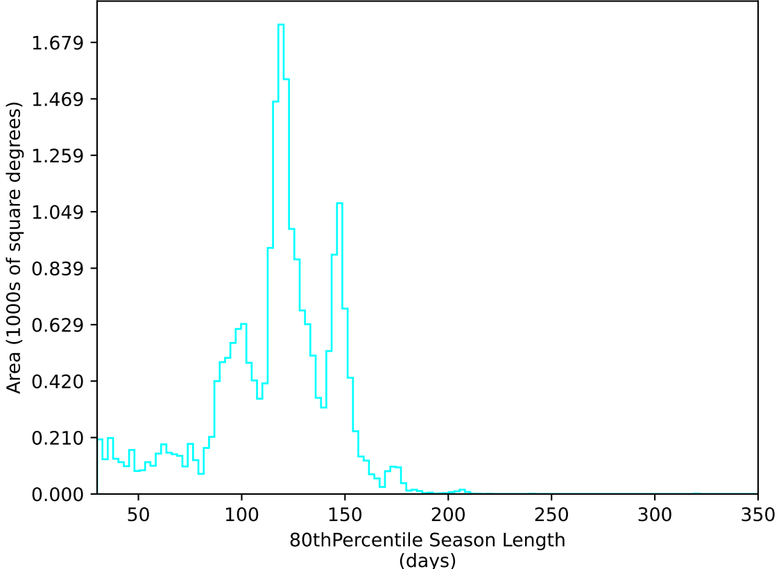
too_elab_r256_d2_griz_v3.4_10yrs All sky u band: 80thPercentile Season Length
