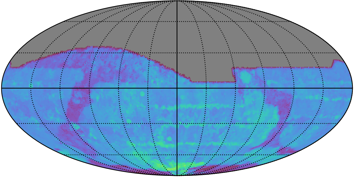
too_elab_r256_d2_griz_v3.4_10yrs All sky i band: 80thPercentile Season Length
