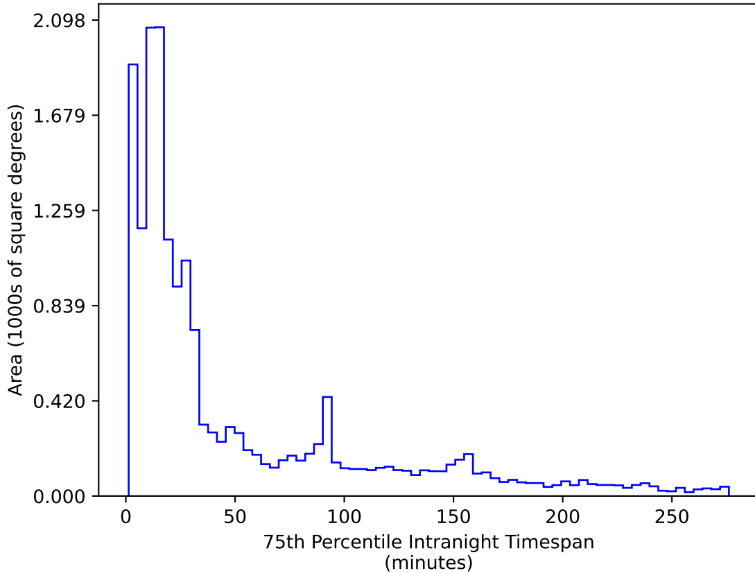
too_elab_r256_d2_griz_v3.4_10yrs WFD r band: 75th Percentile Intranight Timespan
