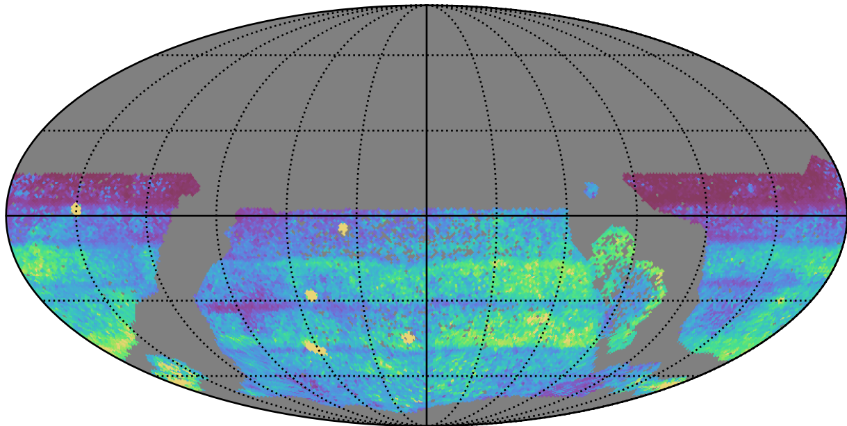
too_elab_r256_d2_griz_v3.4_10yrs WFD all bands: 75th Percentile Intranight Timespan
