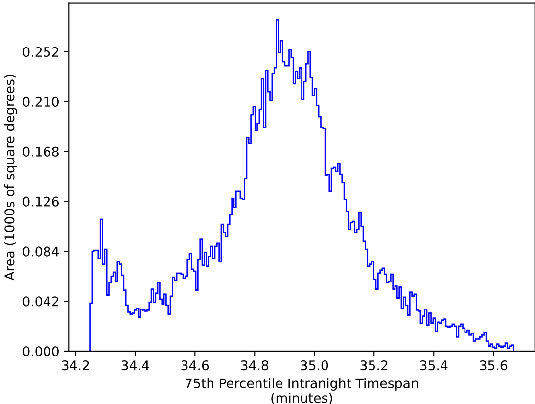
too_elab_r256_d2_griz_v3.4_10yrs WFD: 75th Percentile Intranight Timespan
