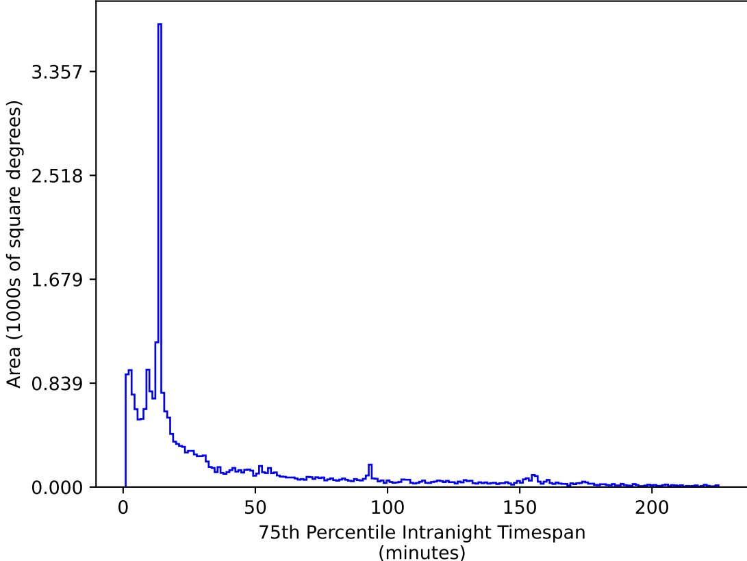
too_elab_r256_d2_griz_v3.4_10yrs All sky z band: 75th Percentile Intranight Timespan
