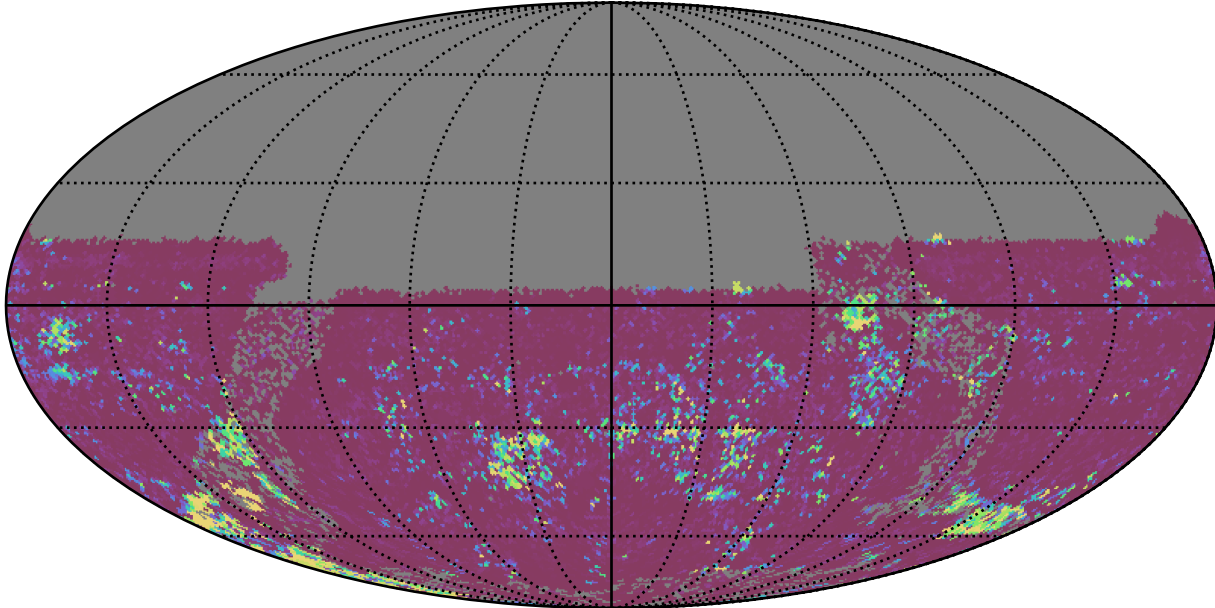
too_elab_r256_d2_griz_v3.4_10yrs All sky u band: 75th Percentile Intranight Timespan
