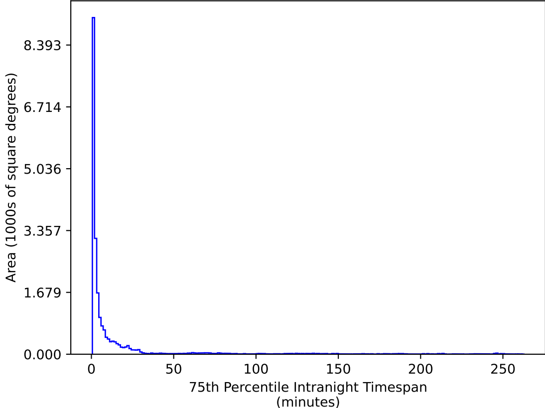
too_elab_r256_d2_griz_v3.4_10yrs All sky u band: 75th Percentile Intranight Timespan
