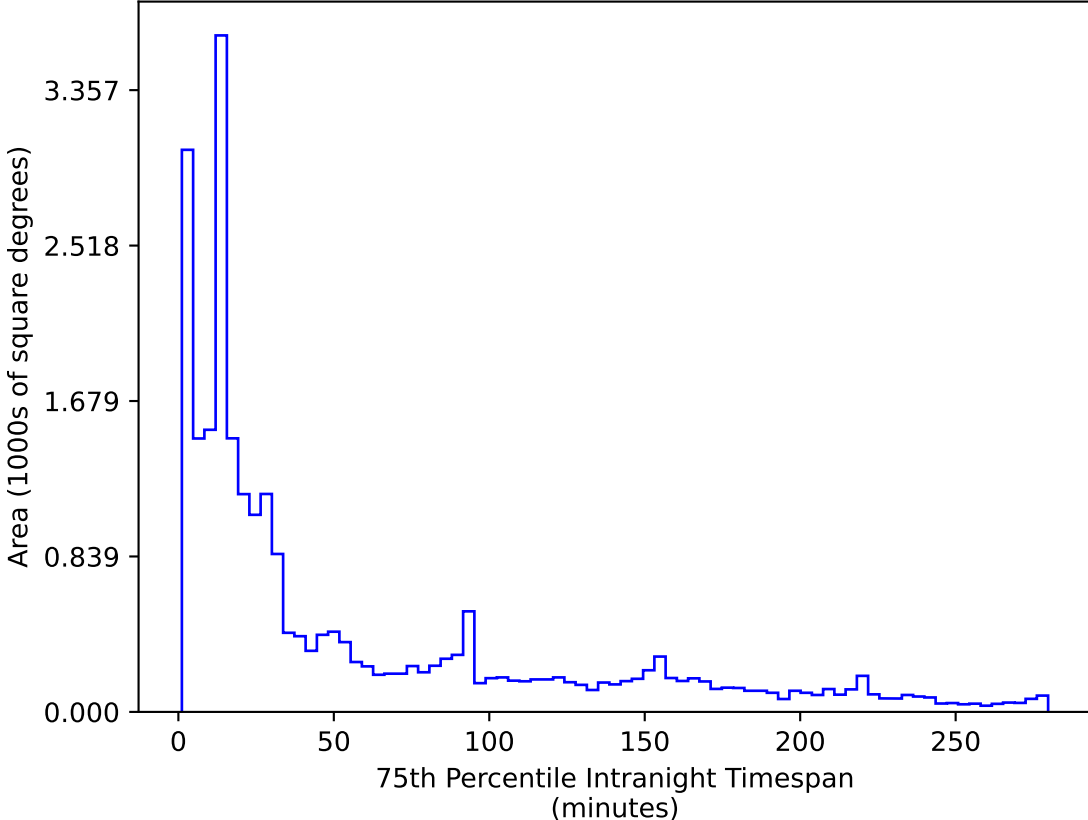
too_elab_r256_d2_griz_v3.4_10yrs All sky r band: 75th Percentile Intranight Timespan
