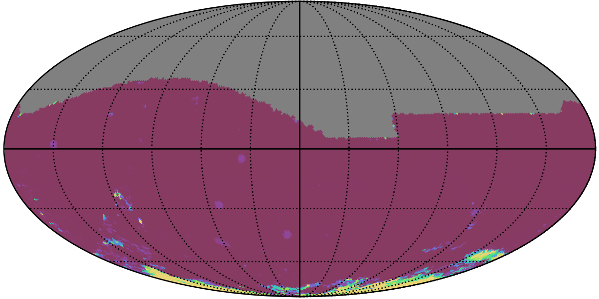
too_elab_r256_d2_griz_v3.4_10yrs All sky iz bands: 75th Percentile Intranight Timespan
