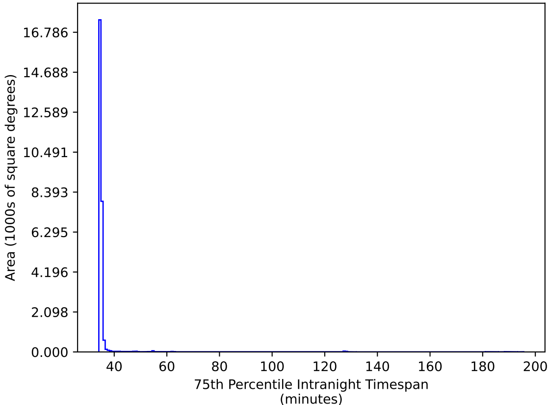
too_elab_r256_d2_griz_v3.4_10yrs All sky iz bands: 75th Percentile Intranight Timespan
