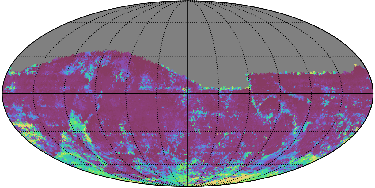
too_elab_r256_d2_griz_v3.4_10yrs All sky i band: 75th Percentile Intranight Timespan
