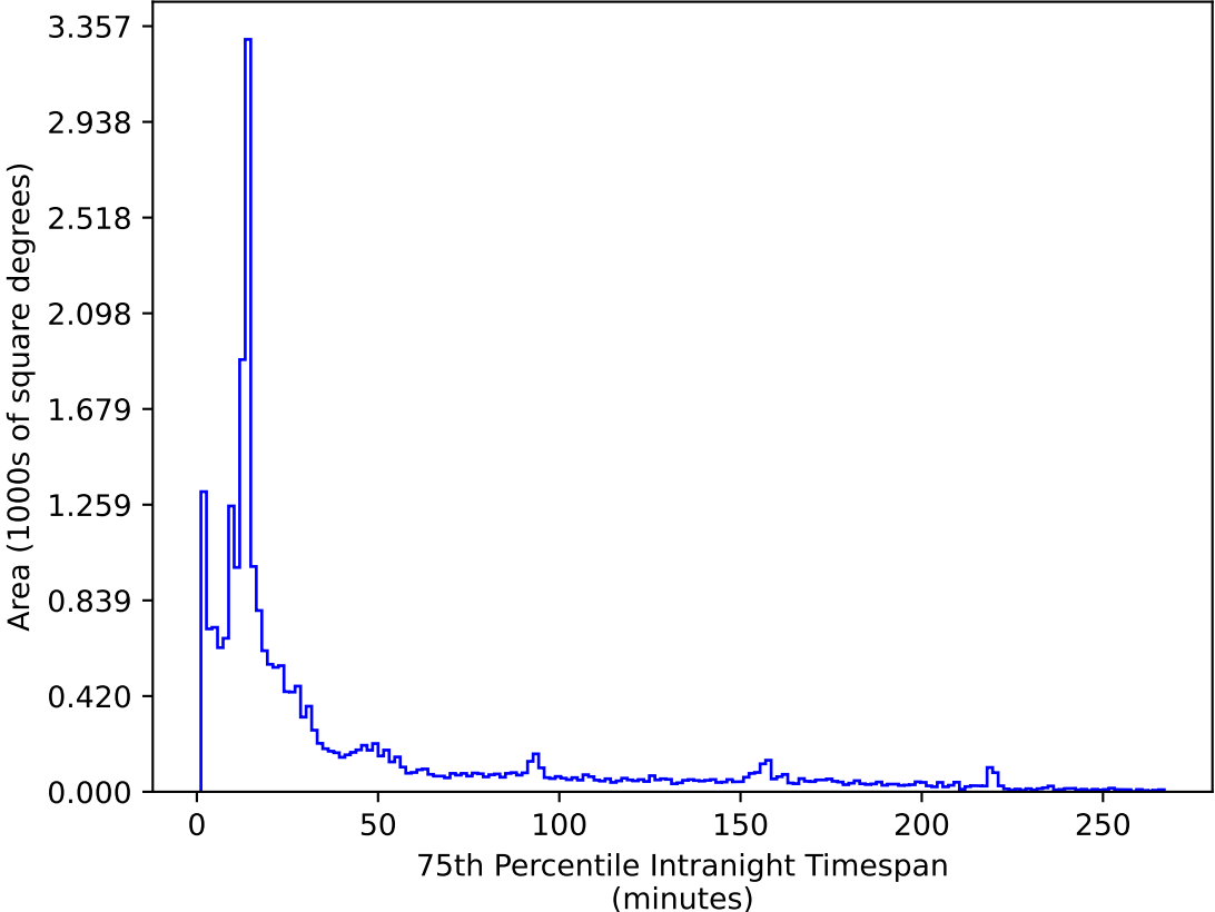
too_elab_r256_d2_griz_v3.4_10yrs All sky i band: 75th Percentile Intranight Timespan
