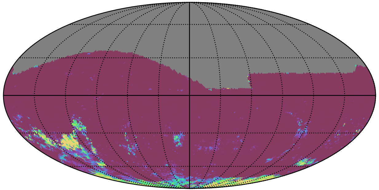
too_elab_r256_d2_griz_v3.4_10yrs All sky gr bands: 75th Percentile Intranight Timespan
