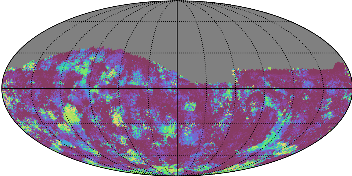
too_elab_r256_d2_griz_v3.4_10yrs All sky g band: 75th Percentile Intranight Timespan
