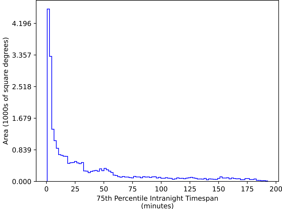
too_elab_r256_d2_griz_v3.4_10yrs All sky g band: 75th Percentile Intranight Timespan
