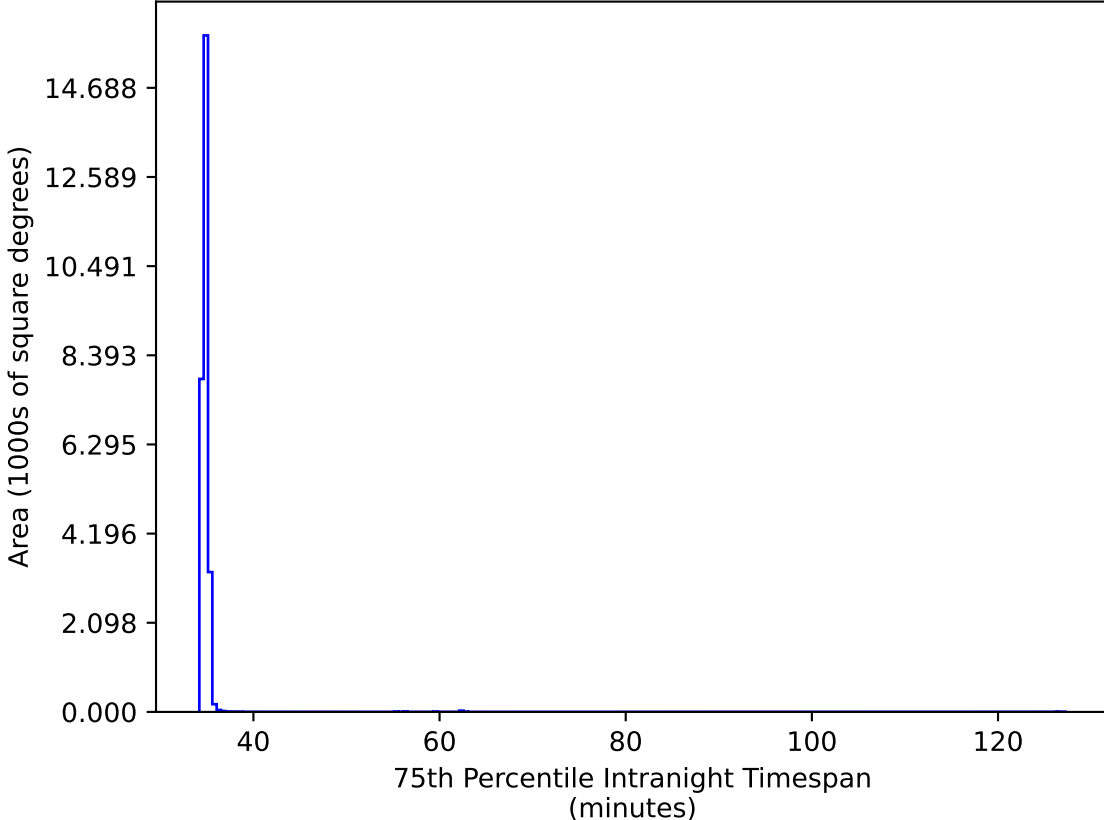
too_elab_r256_d2_griz_v3.4_10yrs All sky all bands: 75th Percentile Intranight Timespan
