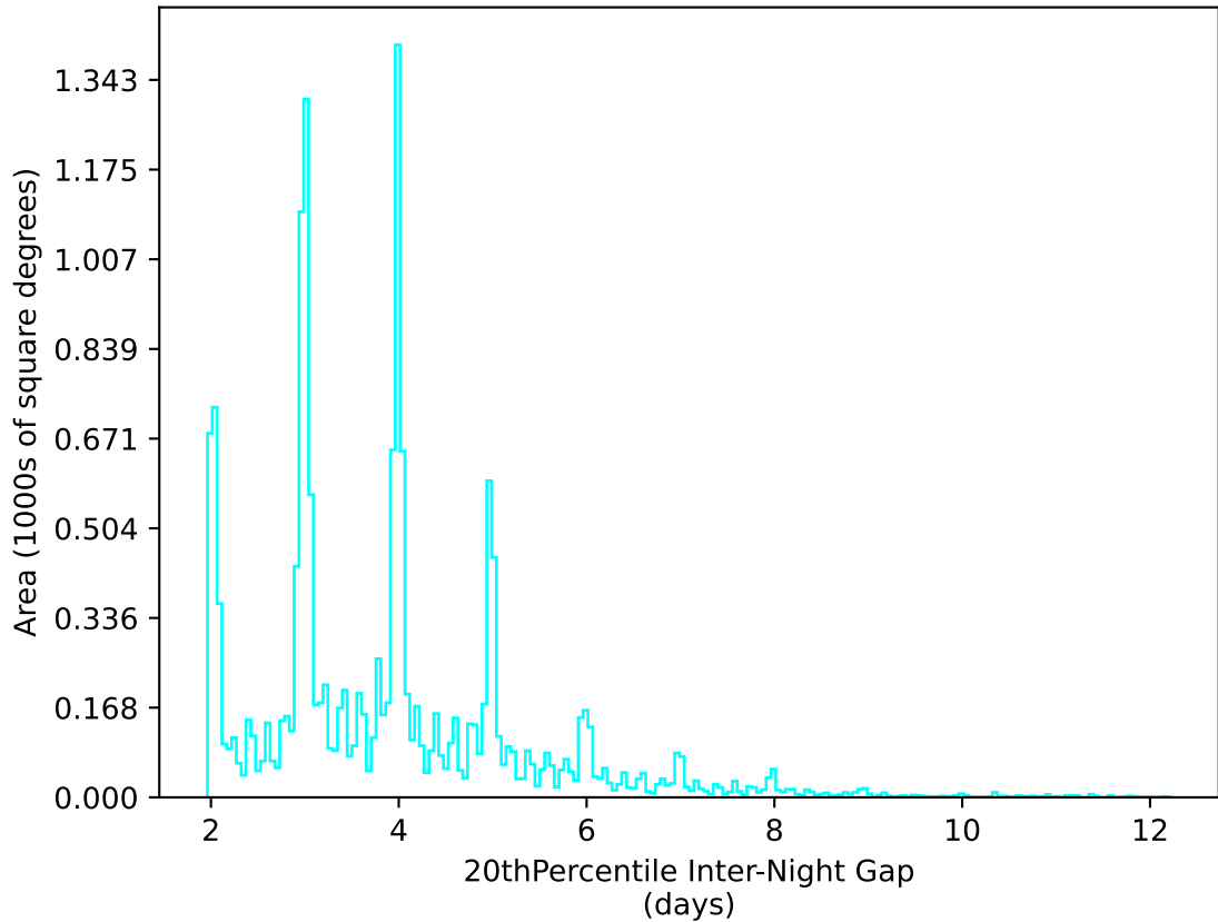
too_elab_r256_d2_griz_v3.4_10yrs WFD u band: 20thPercentile Inter-Night Gap
