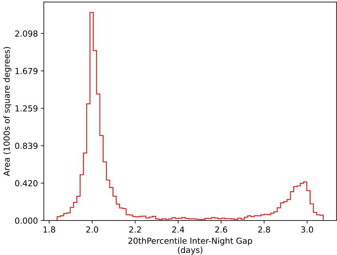
too_elab_r256_d2_griz_v3.4_10yrs WFD i band: 20thPercentile Inter-Night Gap
