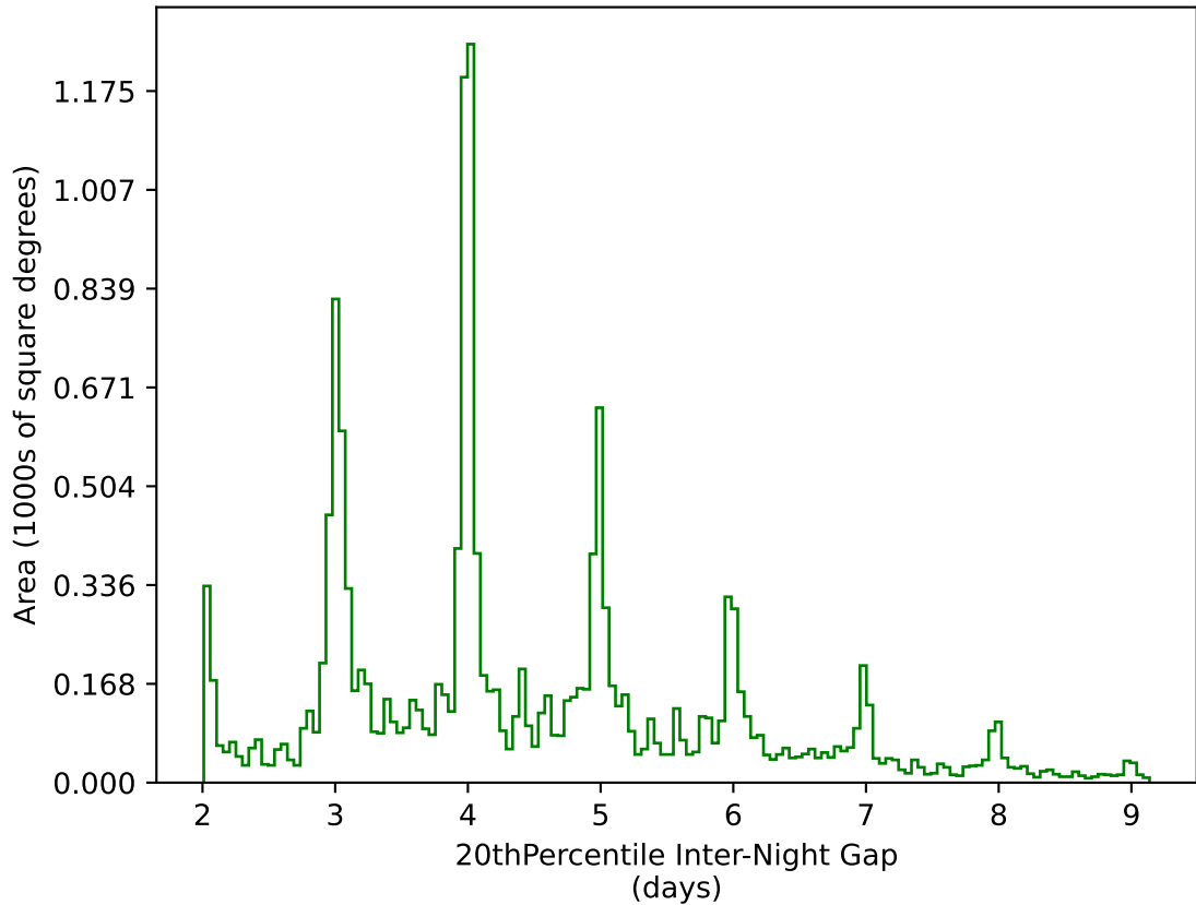
too_elab_r256_d2_griz_v3.4_10yrs WFD g band: 20thPercentile Inter-Night Gap
