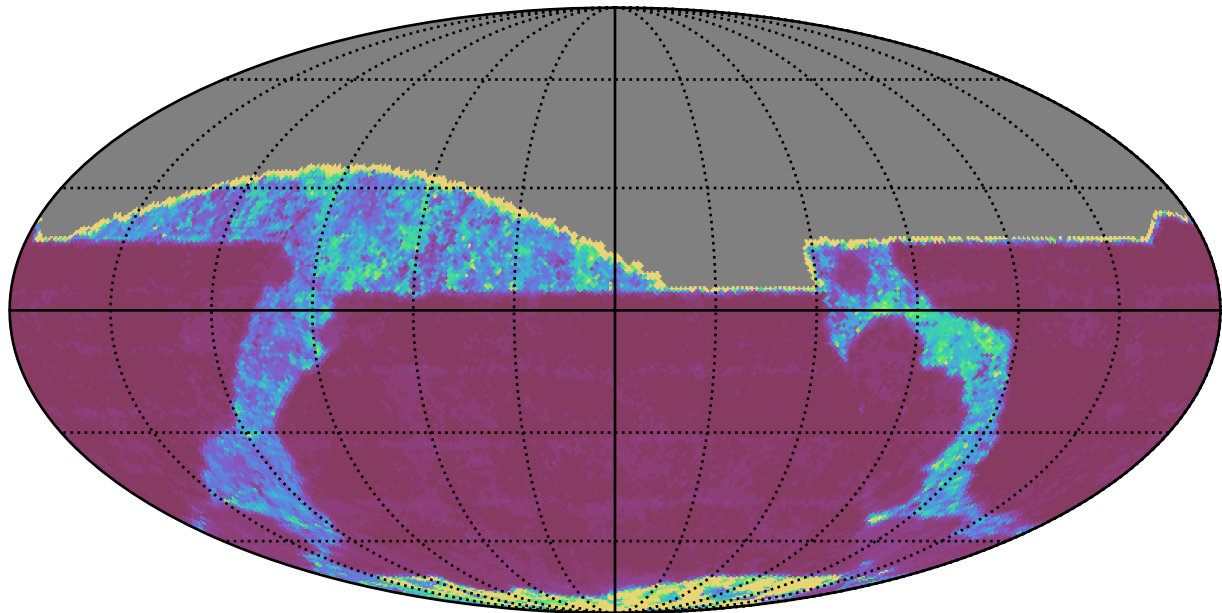
too_elab_r256_d2_griz_v3.4_10yrs All sky i band: 20thPercentile Inter-Night Gap
