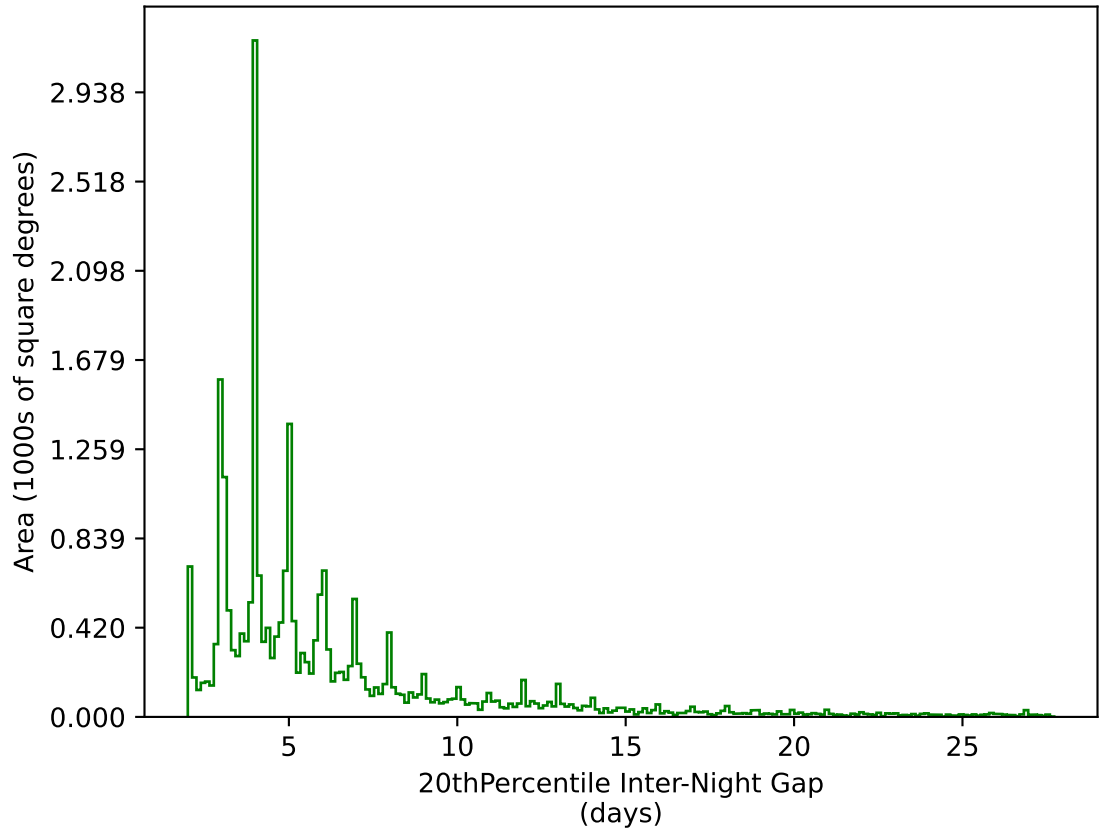
too_elab_r256_d2_griz_v3.4_10yrs All sky g band: 20thPercentile Inter-Night Gap
