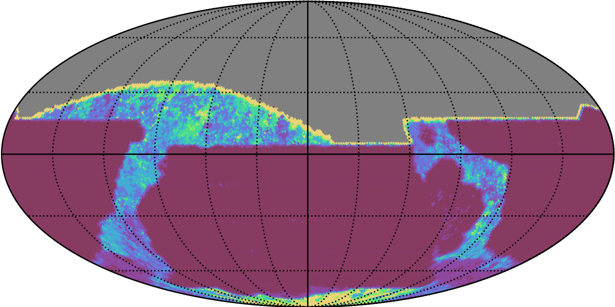
too_elab_r256_d2_griz_v3.4_10yrs All sky all bands: 20thPercentile Inter-Night Gap
