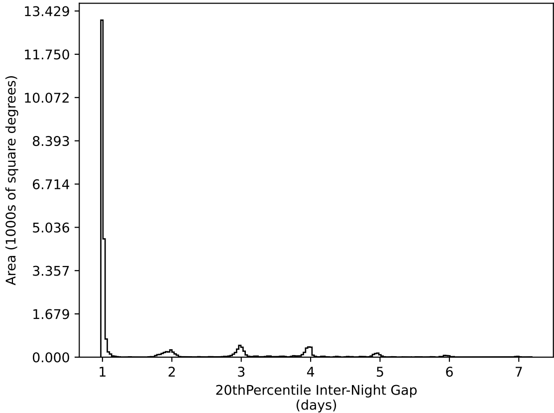
too_elab_r256_d2_griz_v3.4_10yrs All sky all bands: 20thPercentile Inter-Night Gap
