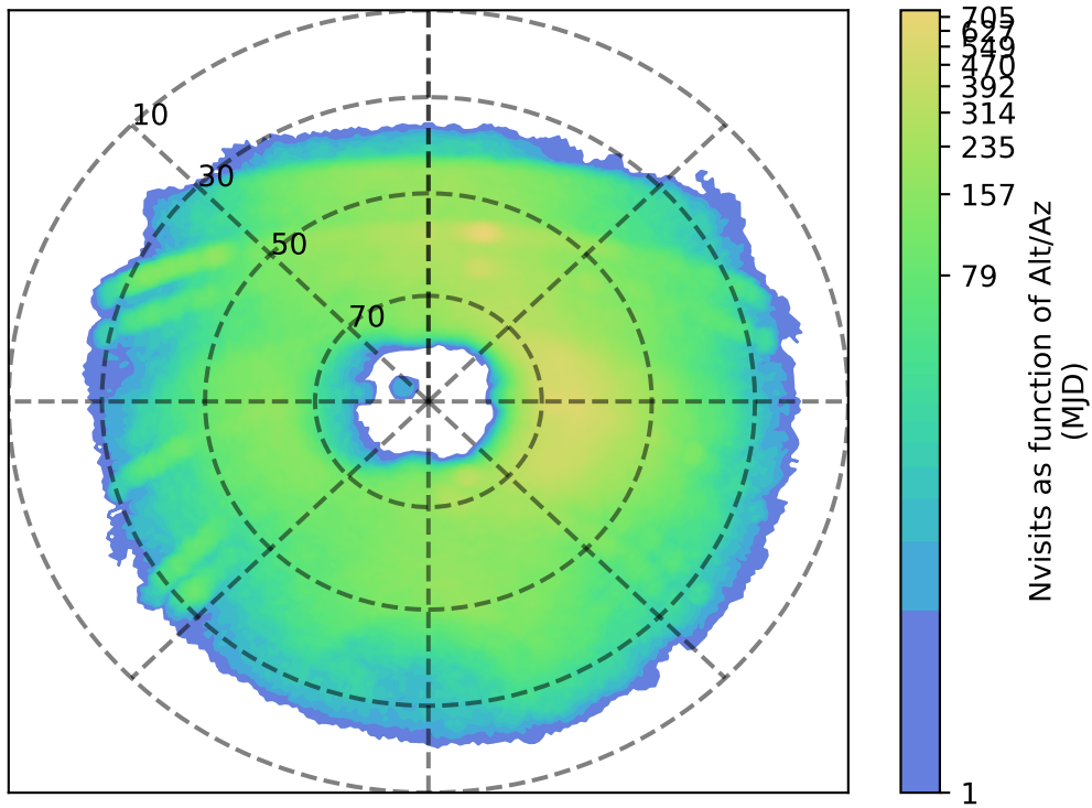
too_elab_r256_d2_griz_v3.4_10yrs u: Nvisits as function of Alt/Az
