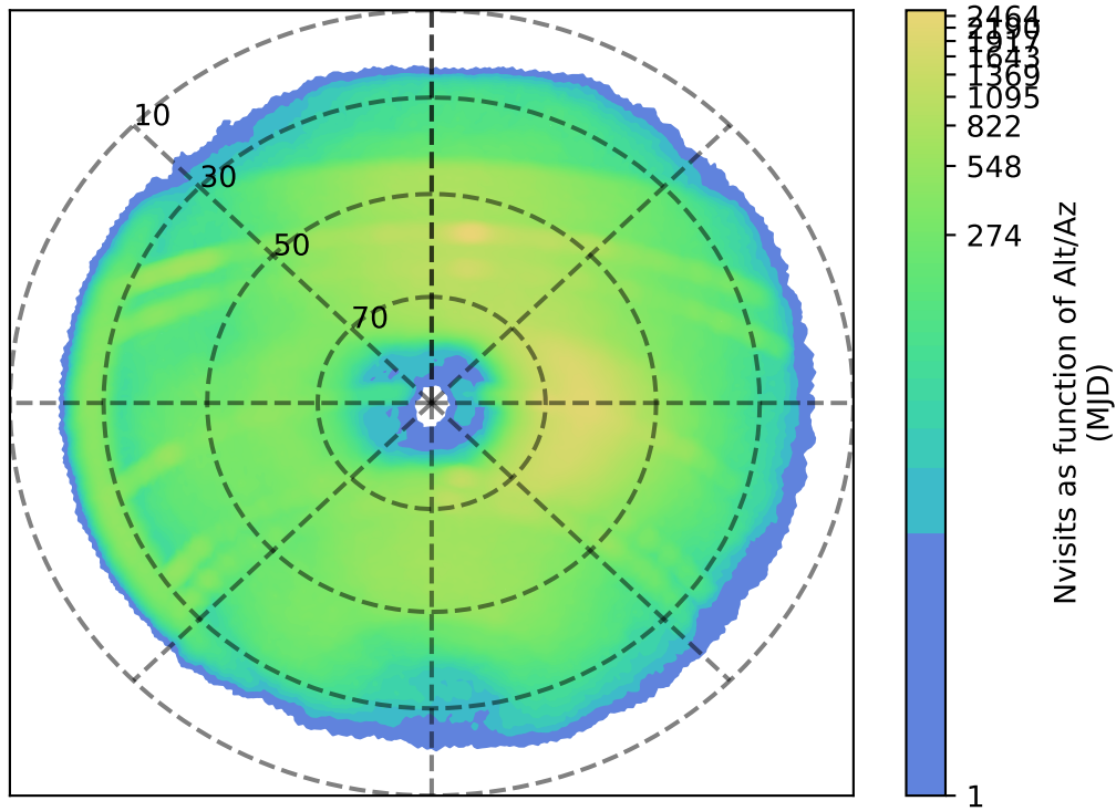
too_elab_r256_d2_griz_v3.4_10yrs r: Nvisits as function of Alt/Az
