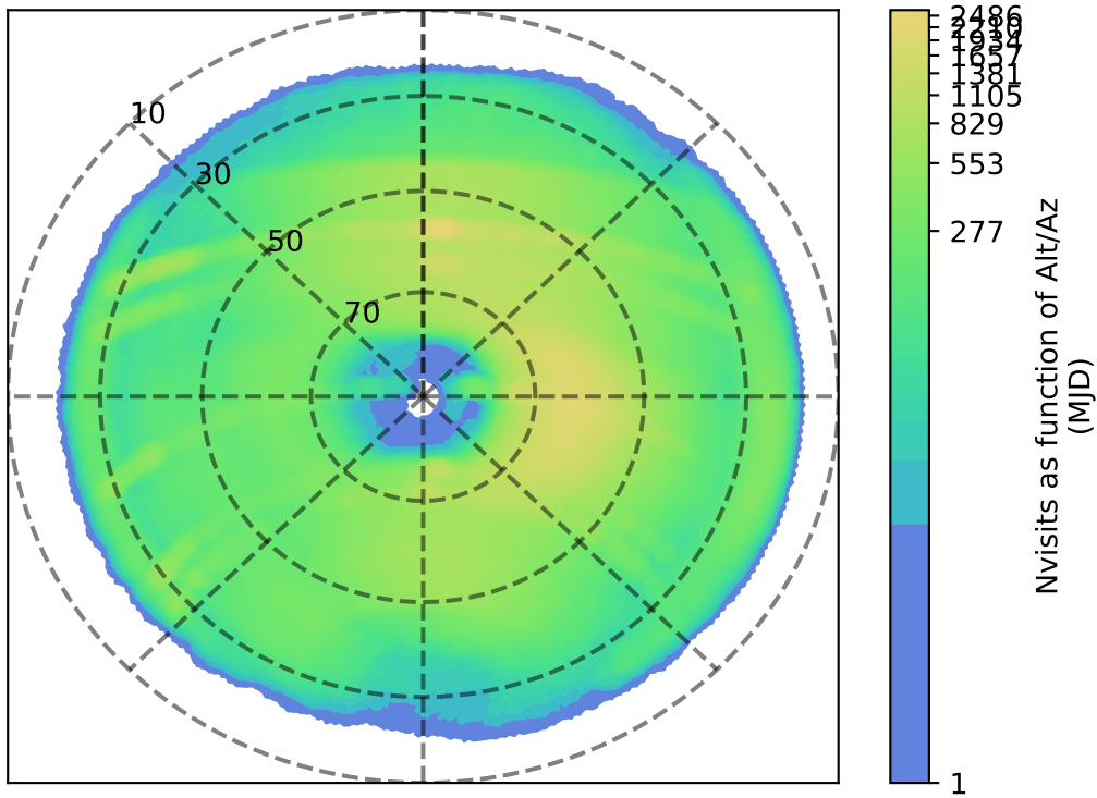
too_elab_r256_d2_griz_v3.4_10yrs i: Nvisits as function of Alt/Az
