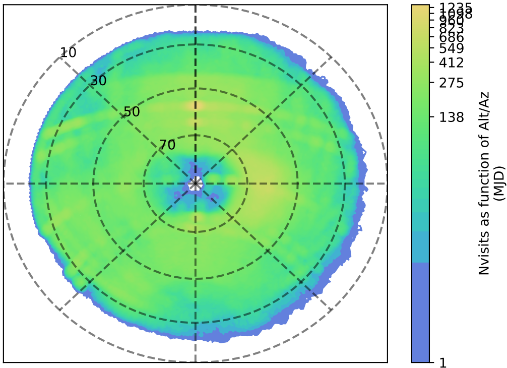
too_elab_r256_d2_griz_v3.4_10yrs g: Nvisits as function of Alt/Az
