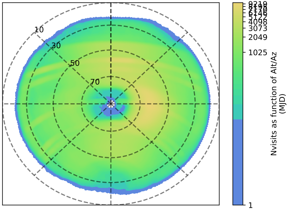
too_elab_r256_d2_griz_v3.4_10yrs : Nvisits as function of Alt/Az
