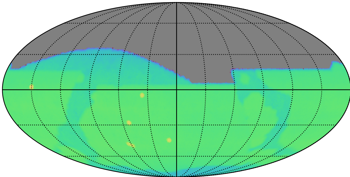
too_elab_r256_d2_griz_v3.4_10yrs : CoaddM5
