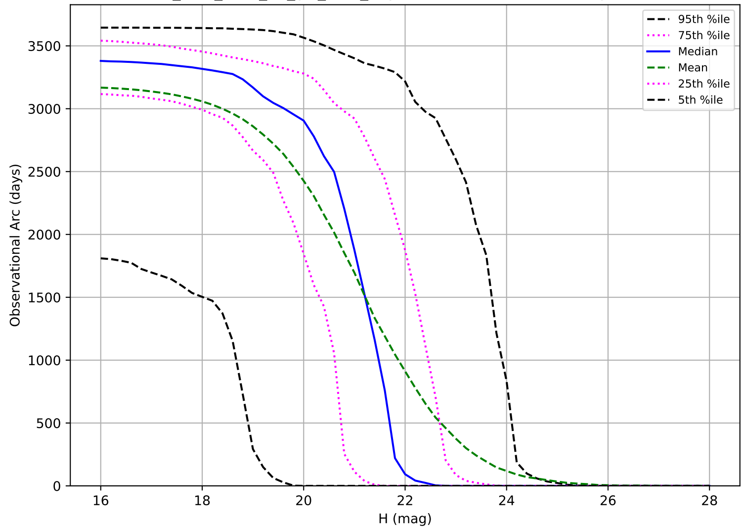
too_elab_r256_d2_giz_v3.4_10yrs: Observational Arc Length NEO
