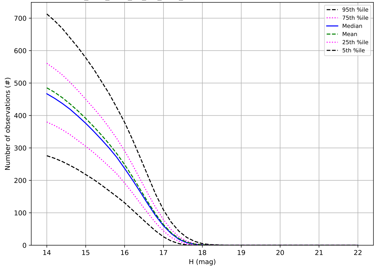
too_elab_r256_d2_giz_v3.4_10yrs: Number of observations Trojan
