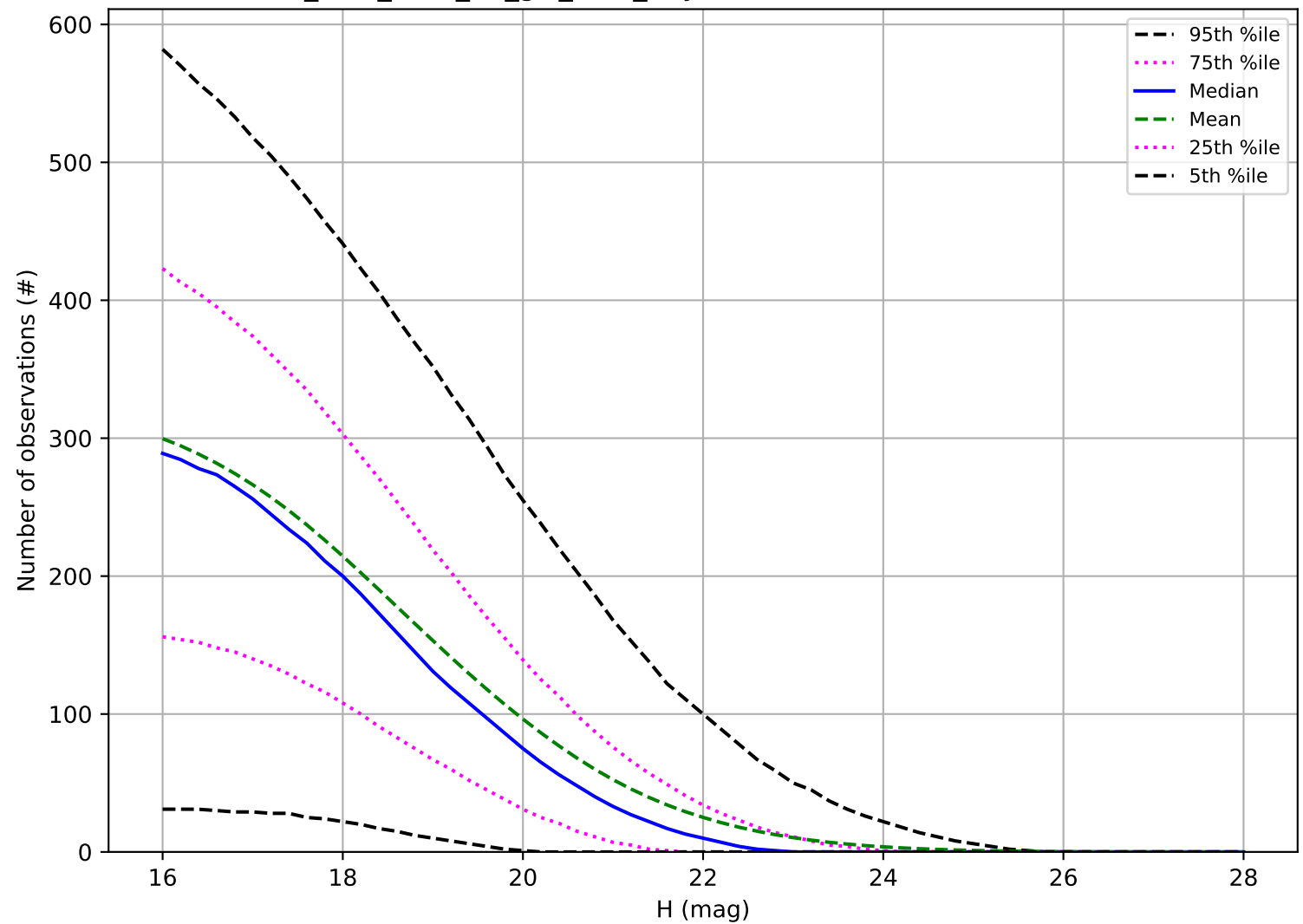
too_elab_r256_d2_giz_v3.4_10yrs: Number of observations NEO
