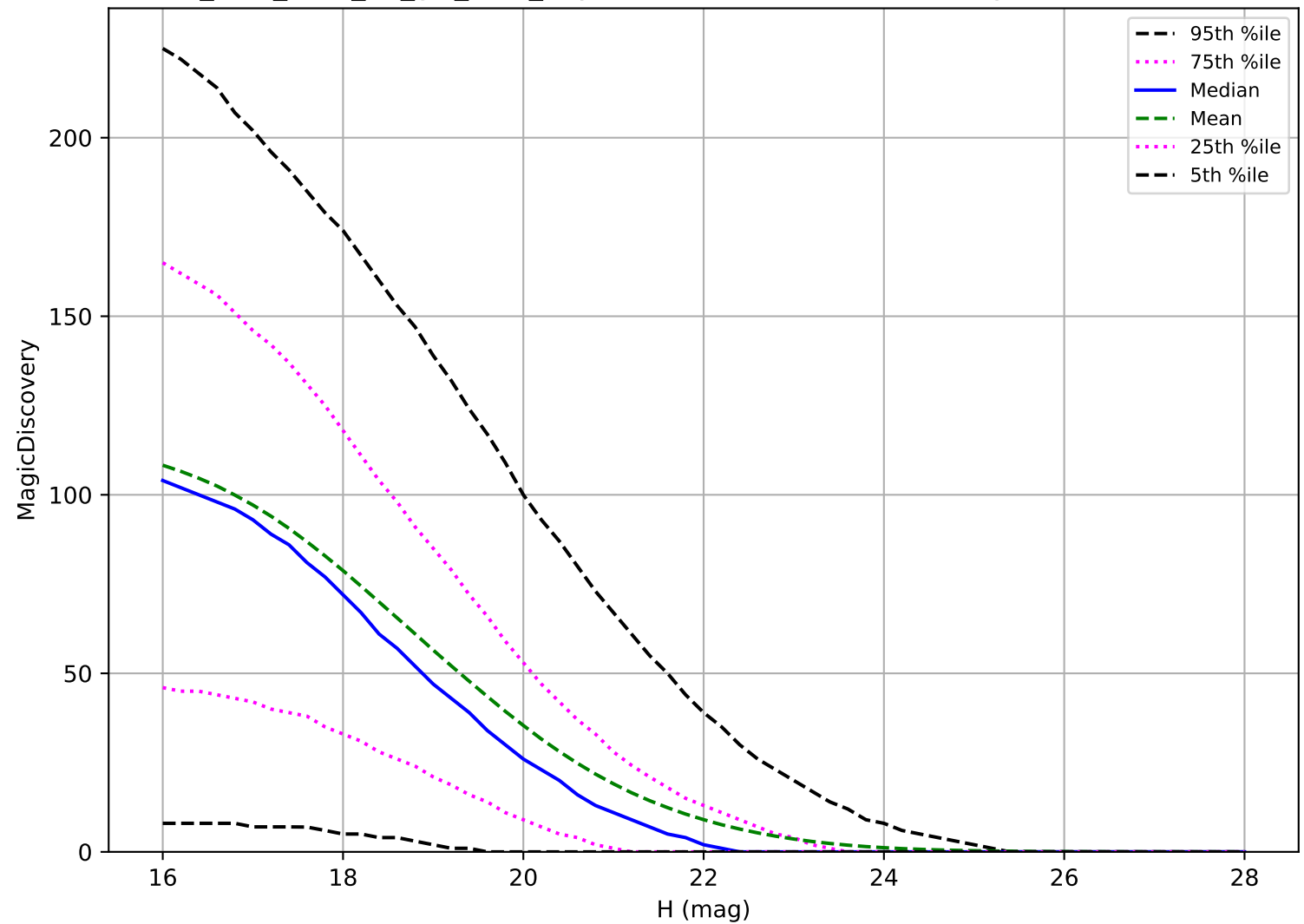
too_elab_r256_d2_giz_v3.4_10yrs: PHA 6 detections in 60 nights detection loss
