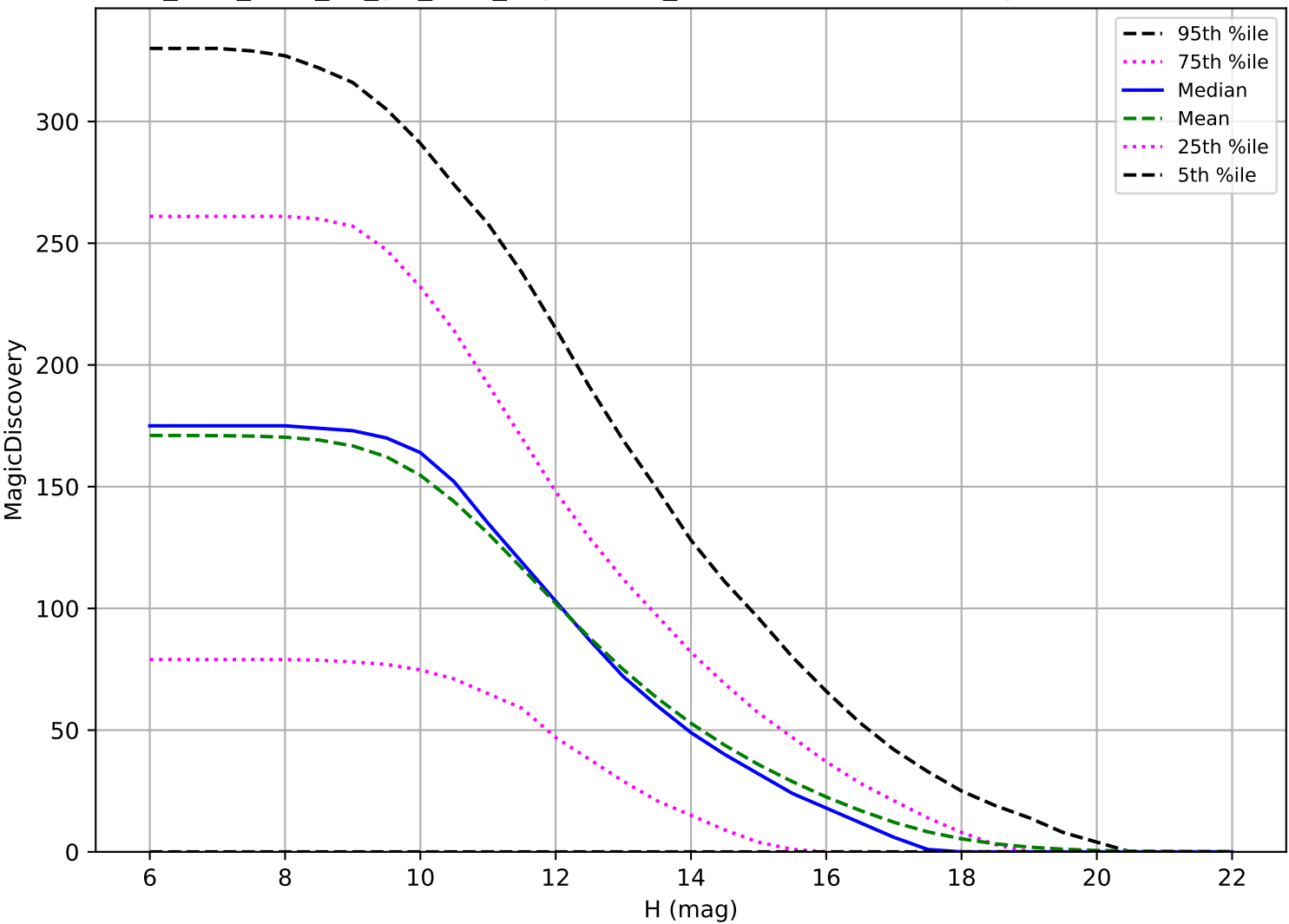
too_elab_r256_d2_giz_v3.4_10yrs: OCC_r5 6 detections in 60 nights detection loss
