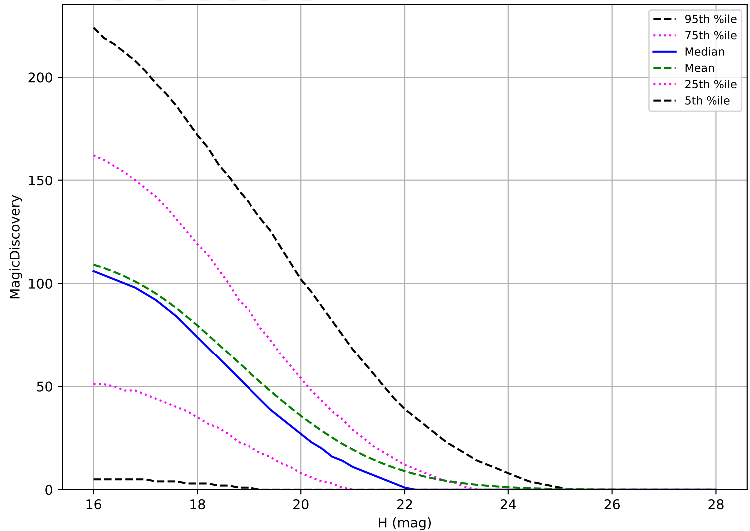
too_elab_r256_d2_giz_v3.4_10yrs: NEO 6 detections in 60 nights detection loss
