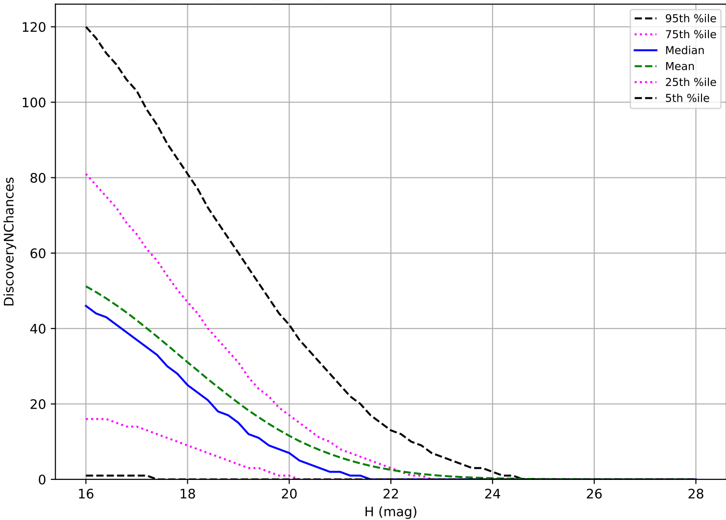
too_elab_r256_d2_giz_v3.4_10yrs: PHA 3 pairs in 15 nights detection loss
