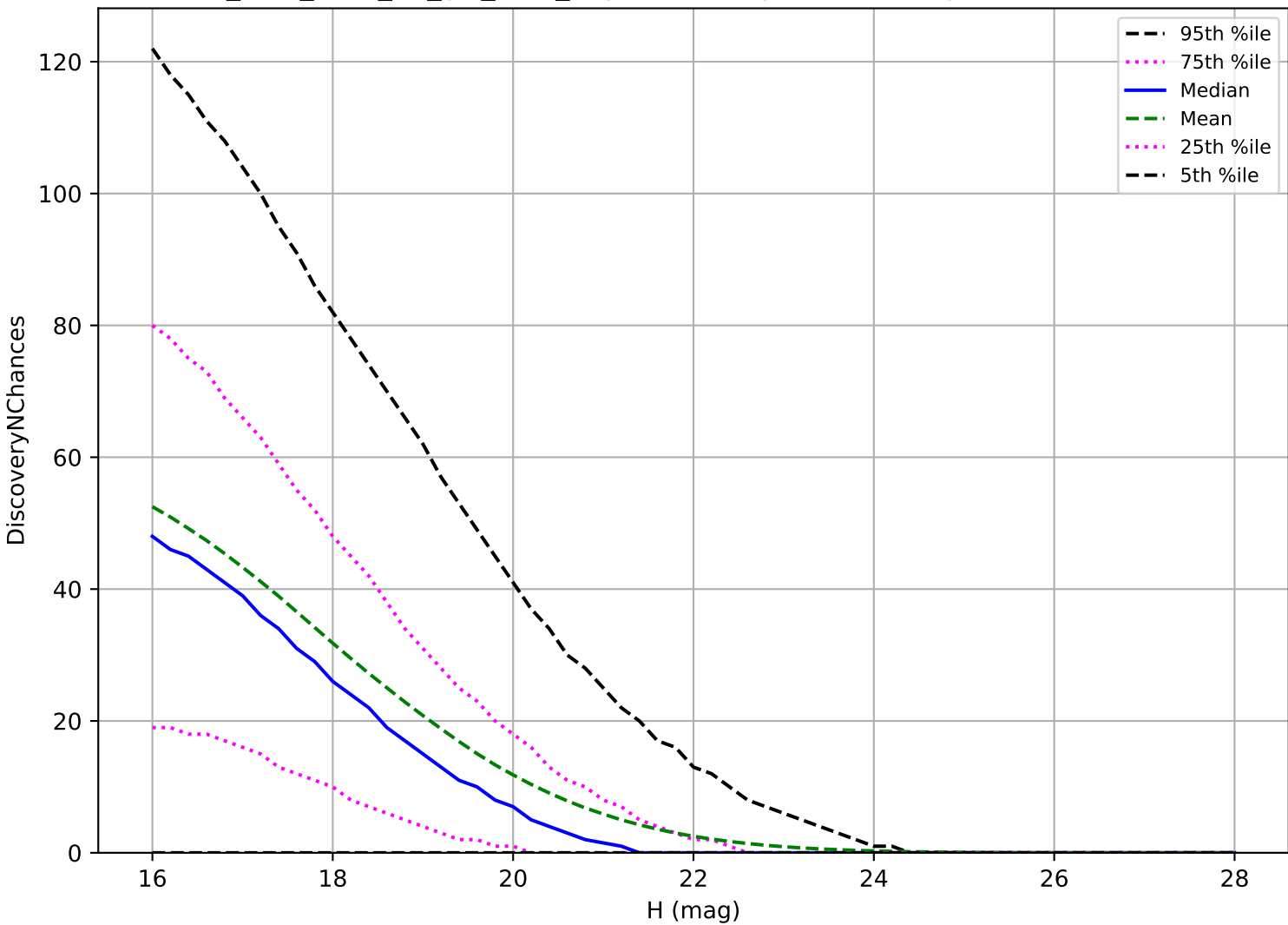
too_elab_r256_d2_giz_v3.4_10yrs: NEO 3 pairs in 15 nights detection loss
