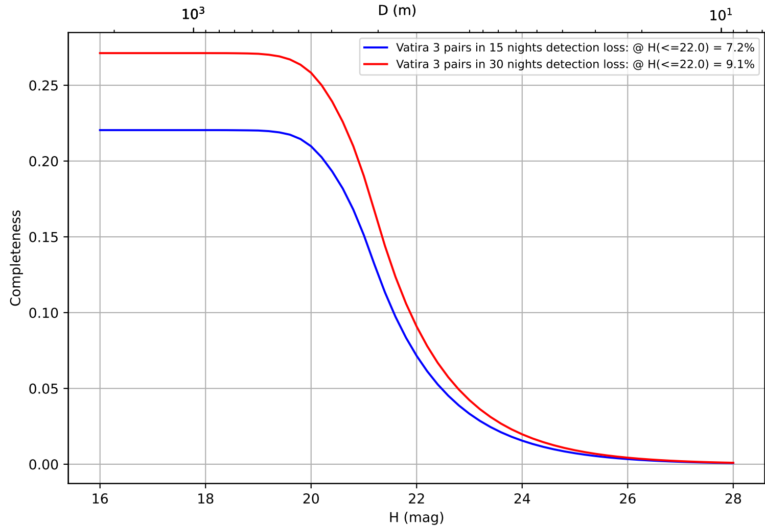
too_elab_r256_d2_giz_v3.4_10yrs: CumulativeCompleteness
