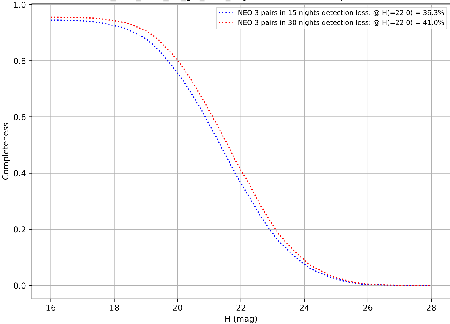
too_elab_r256_d2_giz_v3.4_10yrs: DifferentialCompleteness
