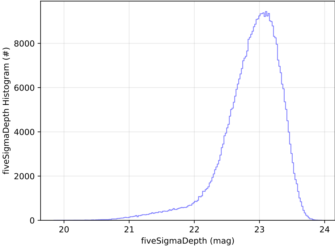
too_elab_r256_d2_giz_v3.4_10yrs z: fiveSigmaDepth Histogram
