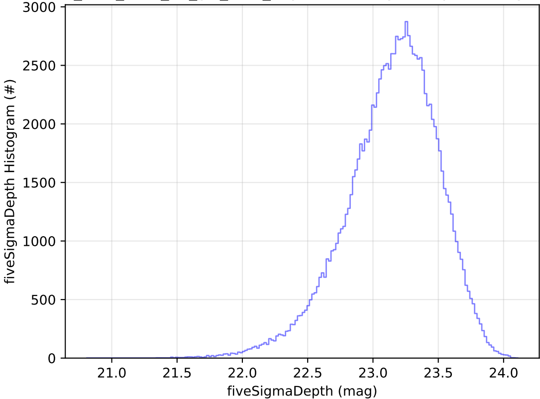
too_elab_r256_d2_giz_v3.4_10yrs u: fiveSigmaDepth Histogram
