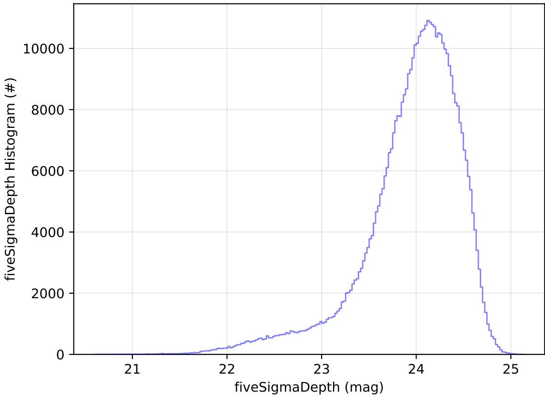
too_elab_r256_d2_giz_v3.4_10yrs r: fiveSigmaDepth Histogram
