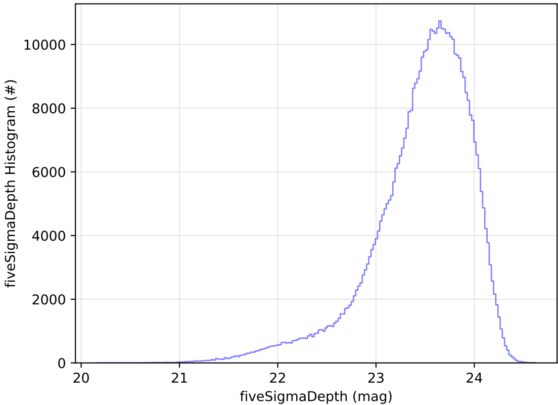
too_elab_r256_d2_giz_v3.4_10yrs i: fiveSigmaDepth Histogram
