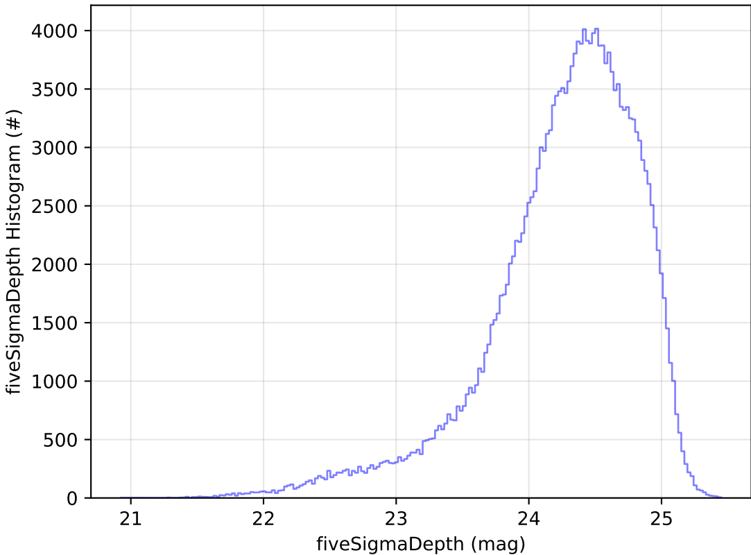
too_elab_r256_d2_giz_v3.4_10yrs g: fiveSigmaDepth Histogram
