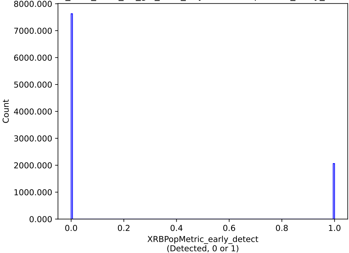
too_elab_r256_d2_giz_v3.4_10yrs : XRBPoMetric_early_detect
