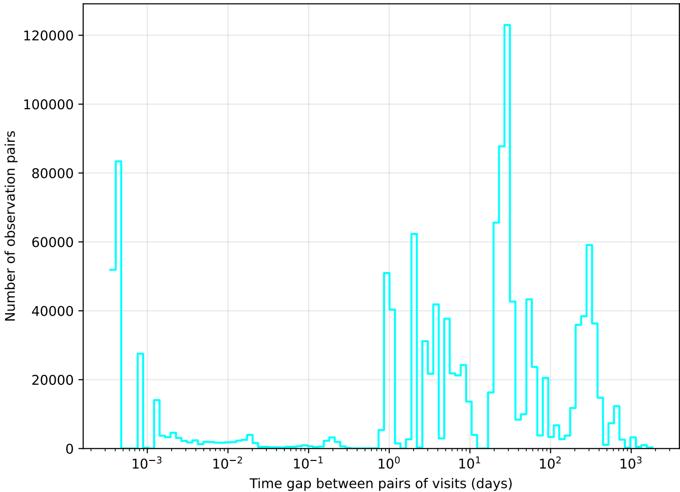
too_elab_r256_d2_giz_v3.4_10yrs u band: Tgaps observationStartMJD
