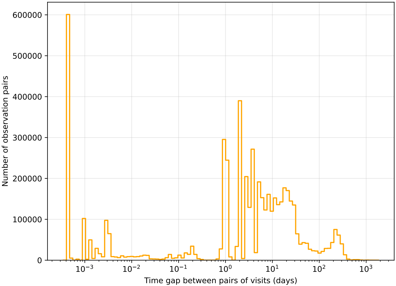
too_elab_r256_d2_giz_v3.4_10yrs r band: Tgaps observationStartMJD
