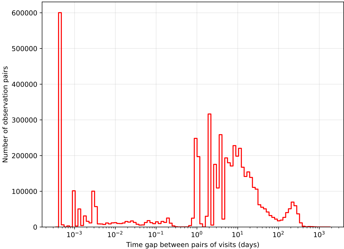
too_elab_r256_d2_giz_v3.4_10yrs i band: Tgaps observationStartMJD
